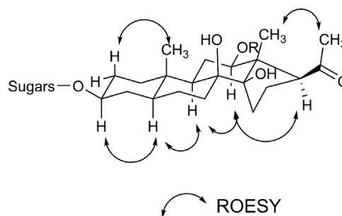
Fig. 3. Selected ROESY dipolar interactions observed for sullivantoside A ( 1 ).
