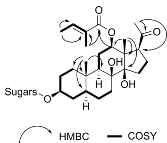
Fig. 2. Selected HMBC and ^1H -COSY correlations observed for sullivantoside A ( 1 ).
