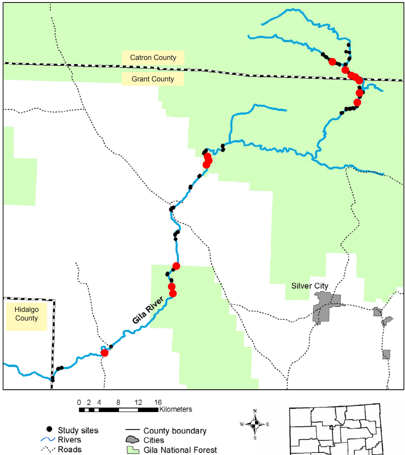
Figure 40. Collection sites (large red dots) for Crotalus molossus along the Gila River.
